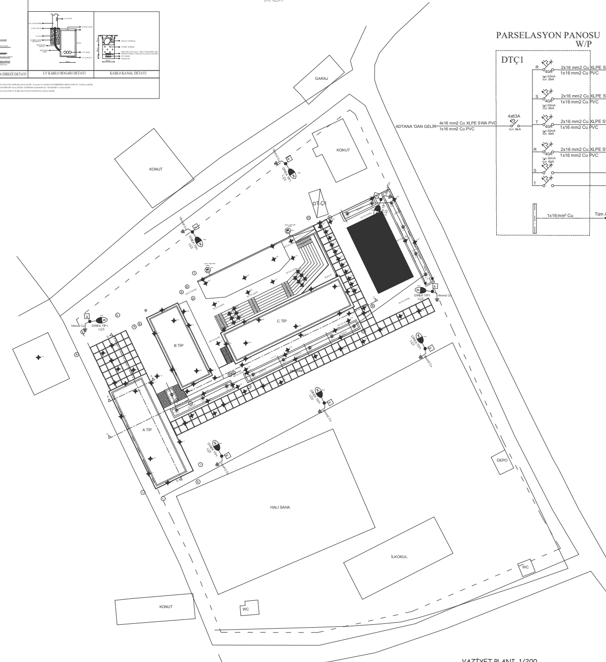
VAZİYET PLANI 1/200
